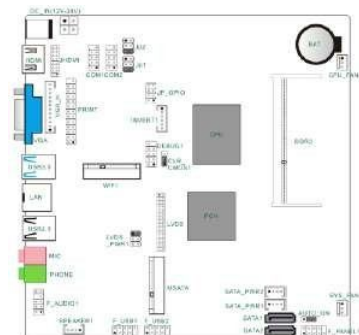
Intel® Core™ i3-3110M Motherboard
